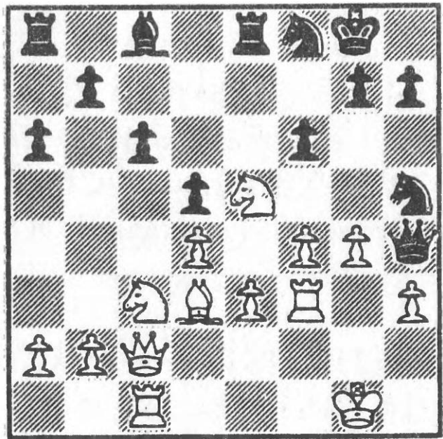
494 After 17...f6
